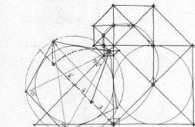
DIMINISHING GOLDEN TRIANGLES
