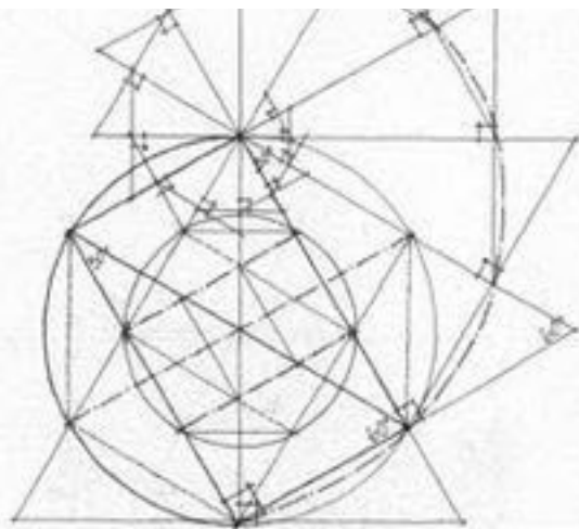
DIMINISHING ROOT 5 RECTANGLES AND TRIANGLES
